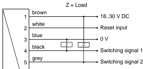
Connection example: PNP NPN
